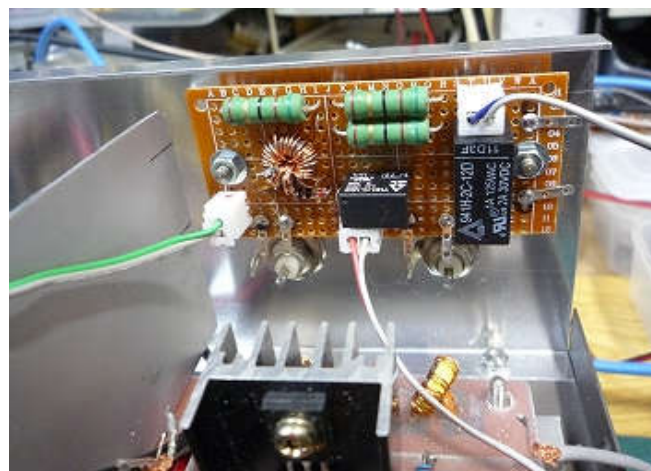
(12) SW取付け
